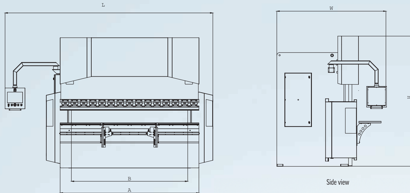
Front view
